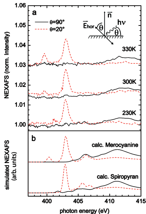
Figure 7. (a) Experimental N K-edge absorption spectra of 1 ML of spiropyran on Au(111), taken during a heating sequence from 230 to 330 K (simultaneously with the data in Figure 4). Continuous black (dashed red) lines correspond to spectra acquired at 90° normal (20° grazing) X-ray incidence. The photon energy resolution was 130 meV. The inset explains the experimental geometry, including the light incidence angle \theta , the sample normal \mathbf{n} , and the polarization vector \vec{E}_{\text{hor}} . The spectra have been shifted vertically for clarity. (b) Calculated NEXAFS spectra for the free SP and MC molecules. For the calculated spectra, the angle of light incidence [90° (continuous black) and 20° (dashed red)] was defined with respect to the molecular plane of the nitrobenzene moiety. 28
