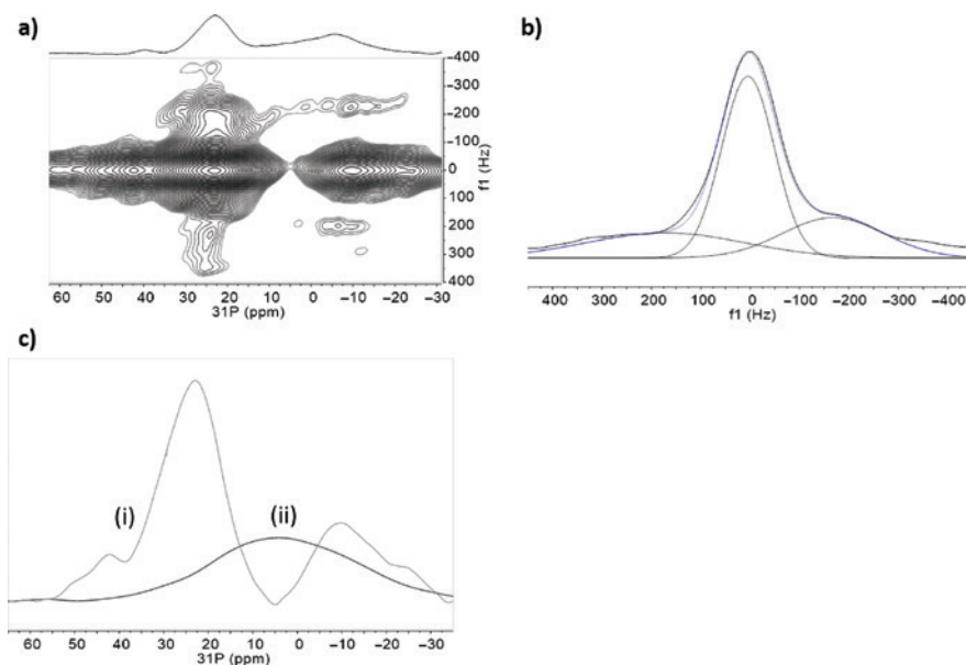
Fig. 2: 2D spectra of Si-PB-Ir-75: (a) ^{31}\text{P} J-resolved spectrum with ( f_1 ) J-coupling in Hz and ( f_2 ) ^{31}\text{P} 1D spectrum. (b) Vertical slice of the ^{31}\text{P} J-resolved spectrum extracted at 23 ppm. (c) Horizontal slice of the ^{31}\text{P} J-resolved spectrum extracted at 0 Hz which represents signals showing no J-couplings (i), overlaid with 1D ^{31}\text{P} inadequate spectrum which represents signals showing J-couplings (ii).
