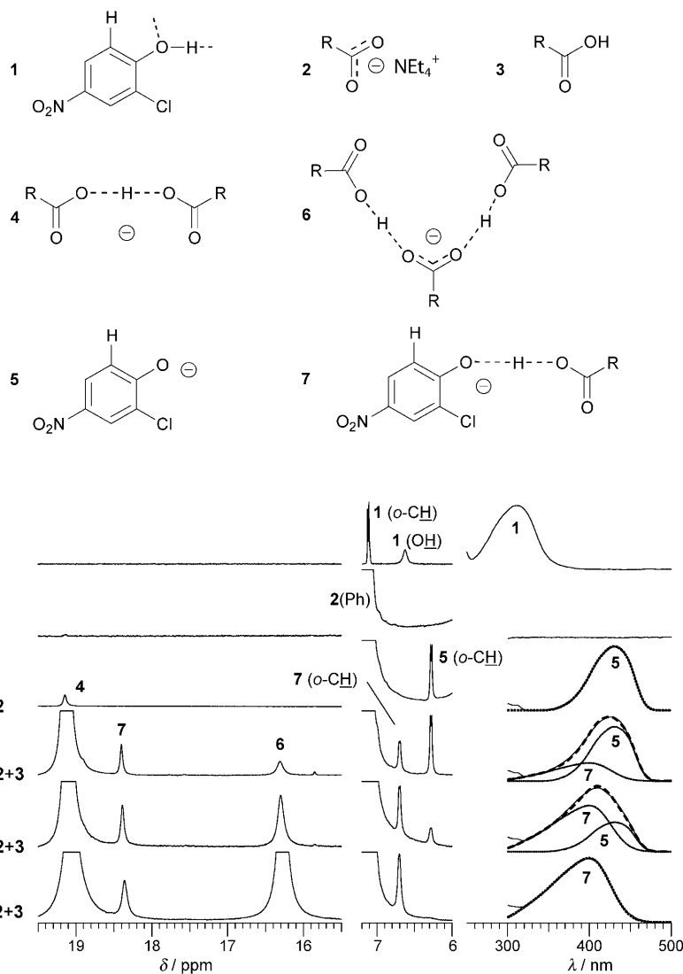
Figure 2. Combined ^1\text{H} NMR (left) and UV/Vis (right) spectra of 1 – 3 dissolved in \text{CD}_2\text{Cl}_2 recorded at 175 K; \text{R} = \text{PhCH}_2\text{CH}_2 ; dotted lines in UV/Vis spectra indicate the deconvolution of the bands. Concentrations of 1/2/3 in mM: A) 1:0:0, B) 0:29:0, C) 1:28:0, D) 1:23:17, E) 1:22:19, F) 1:21:23.
