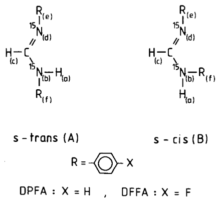
Fig. 2. Atom labeling of ^{15}\text{N},^{15}\text{N}' -di-(4-fluorophenyl)-formamidines in the s -cis and the s -trans form.
