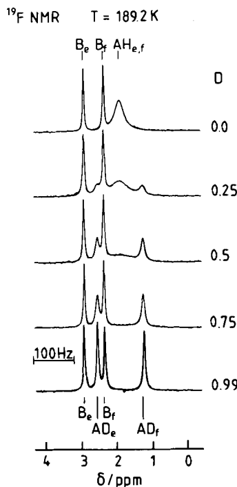
Fig. 5. Superposed experimental and calculated ^{19}\text{F}\{-^1\text{H}\} -NMR spectra of 0.02 molar solutions of DFFA in THF as a function of the deuterium fraction D . For the explanation of the atom labeling see Figure 2. The pseudo first order rate constants of the proton exchange are labeled as k_2^{\text{LM}} , LM=HH, HD, DD. In the fitting procedure, k_2^{\text{DD}} was set constant to a value of 3 \text{ s}^{-1} (see Figs. 6 and 7); by simultaneous non-linear regression analysis of all spectra we obtained k_2^{\text{HH}} = 700 \text{ s}^{-1} and k_2^{\text{HD}} = 33 \text{ s}^{-1} . The linewidth in the absence of exchange W_0 \approx 5 \text{ Hz} was obtained from the \text{B}_e and \text{B}_f signals.
