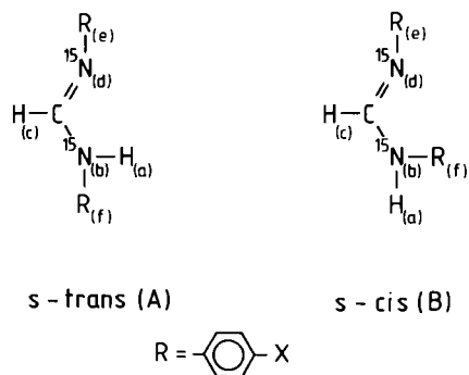
Fig. 2. Atom labeling of ^{15}\text{N},^{15}\text{N}' -di-(fluorophenyl)-formamidines in the s -cis and the s -trans form.
