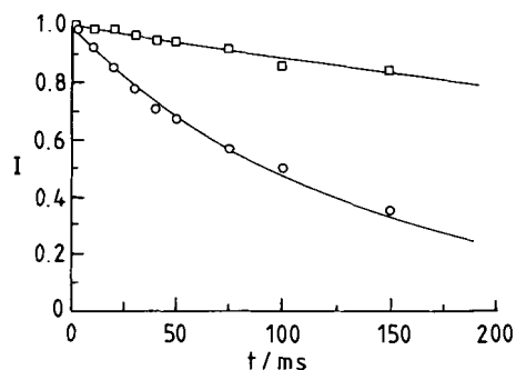
Fig. 7. Analysis of the data in Figure 6. Parameters of the non-linear regression analysis: T_{1\rho}=808 ms and k_2^{\text{DD}}=3.05 \text{ s}^{-1} .
